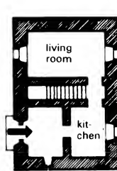
⑭ The stone house (AD 1500): massive walls, to combat enemies/cold, required the same area as the rooms themselves
